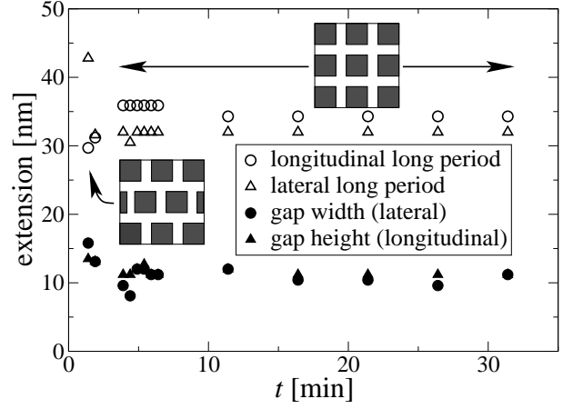
Figure 7: Evolution of the block nanostructure during crystallization at 140°C. Two observed block arrangements are sketched in insets. During the first 3 min the temperature is not yet constant, and the block arrangement ( left inset ) is different from the arrangement ( right inset ) during the isothermal period
