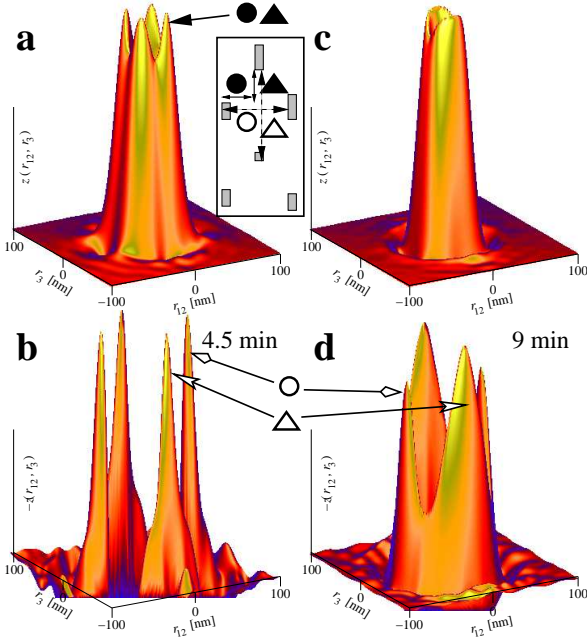
Figure 9: CDFs during the isothermal phase of PP recrystallization at 145°C. Top : positive faces. Bottom : negative faces. After 4.5 min ( a, b ) the initial short-range correlated block structure (cf. Fig. 6) is still visible. Arrows point at the peaks of the CDF. The indicated symbols are related to the curves shown in Fig. 8. The inset shows the relation of the quantities to the simple nanostructure model. After 9 min ( d ) in the shortest-range correlations between neighboring domains have considerably widened
