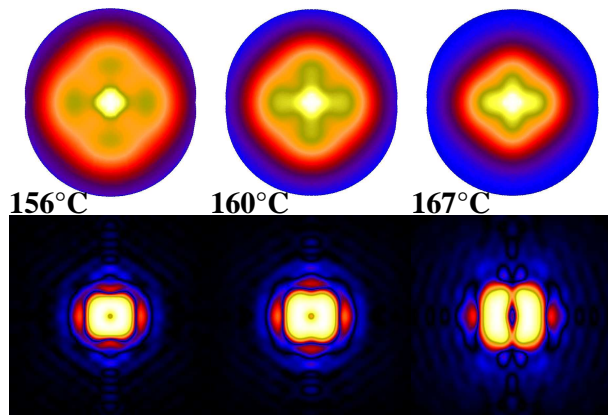
Figure 11: Second melting of PP material previously crystallized at 140°C. Top row: SAXS patterns. Bottom row: CDFs |z(r_{12}, r_3)| . The regions shown are the same as in the corresponding previous figures
