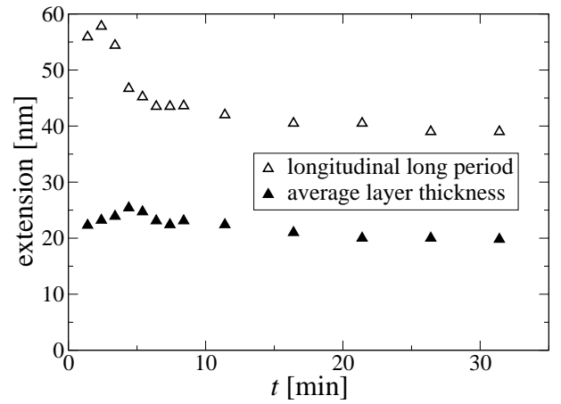
Figure 10: Evolution of the nanostructure during crystallization at 150°C. Lamellae are observed from the beginning of structure formation. Amorphous and crystalline thickness are merged into one broad peak. Filled triangles show the evolution of the position of its maximum
