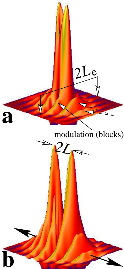
Figure 1: Demonstration of CDF analysis for the simple case of a predominant lamellar system (Melting PP. The function is shown in an interval -100\text{nm} < r_{12}, r_3 < 100\text{nm} ). (a) shows the positive face -z(\mathbf{r}) with the layer peaks visible. 2L_e is the double lateral extension of a single layer. The solid-line arrow indicates a modulation inside the lamella in lateral direction which is typical for a blocky system. The sandwiches of two or three lamellae (broken-line arrows) are not modulated. (b) shows the negative face -z(\mathbf{r}) with the long-period peaks visible. The distance between the two small arrows on top is the double long period. The filled arrows below indicate the fiber direction, r_3
