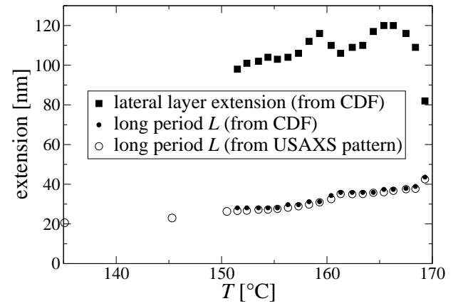
Figure 4: Evolution of nanostructure parameters in hard-elastic PP during heating to the melt. Heating rates: 2^\circ\text{C}/\text{min} above 150^\circ\text{C} ; 20^\circ\text{C}/\text{min} below 150^\circ\text{C}
