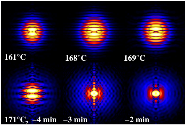
Figure 2: SAXS patterns recorded during the heating and melting of PP (logarithmic intensity scale). Sample temperatures and times before quench to crystallization temperature are indicated. The sensitive region is 0.002 \text{ nm}^{-1} < |s| < 0.05 \text{ nm}^{-1} in reciprocal space. s_3 -direction (i.e. orientation axis, fiber axis, meridian) is vertical
