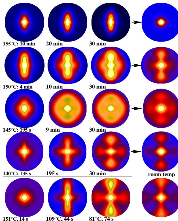
Figure 5: Oriented quiescent crystallization of PP from a melt of 171°C quenched to different crystallization temperatures as a function of time. Pseudo-color images of the measured SAXS patterns (logarithmic intensity scale). The rightmost column shows the ultimate nanostructure after cooling to room temperature. Bottom row: Nonisothermal crystallization (rapid direct quench)
