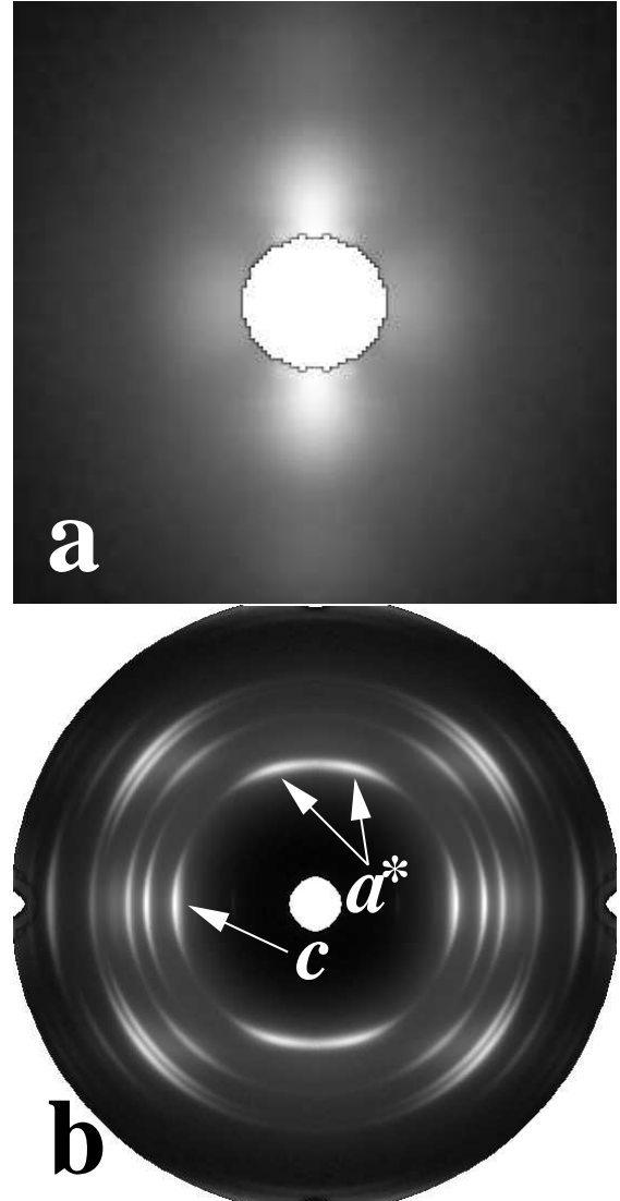
Figure 12: Test of the WAXS orientation related to a recrystallized material showing (a) the SAXS cross pattern. The WAXS pattern (b) shows the same bimodal orientation as the original material with plain lamellar SAXS. The (110) reflections related to c -axis oriented crystals and a^* -axis oriented crystals are indicated by arrows
